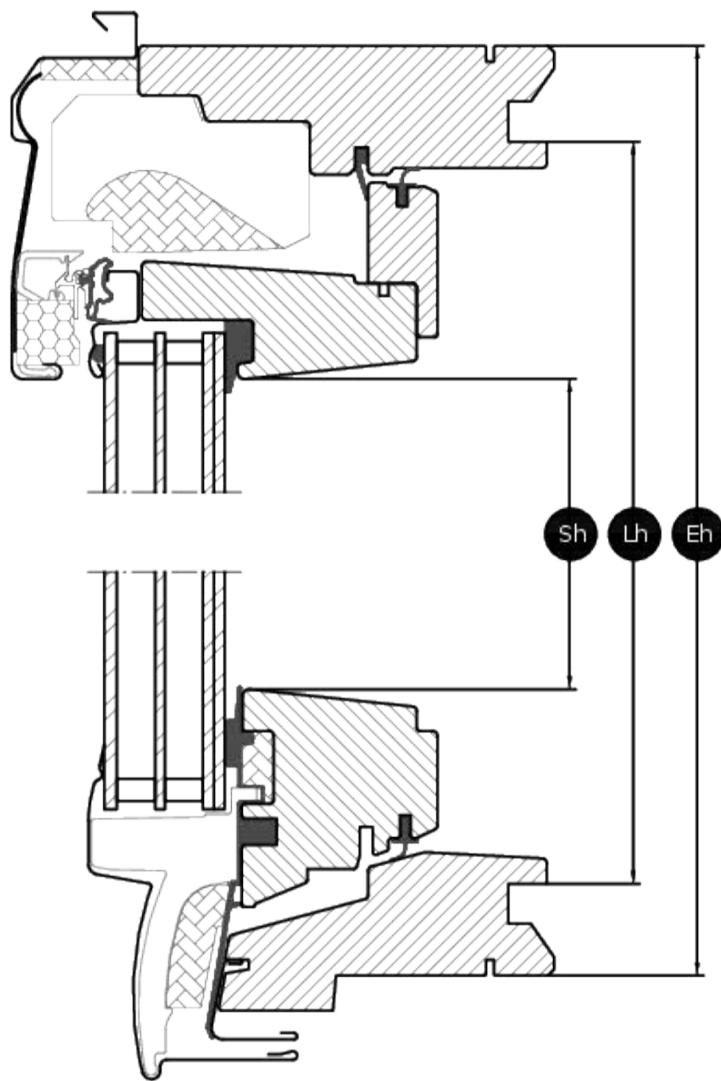
Middel section Fixed window
