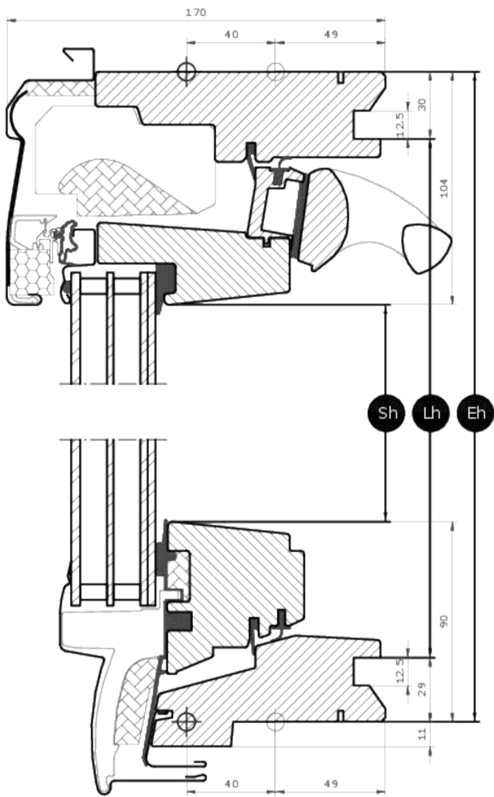
Side sections Pivot windows
